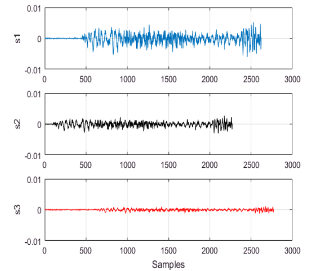
Misaligned signals
